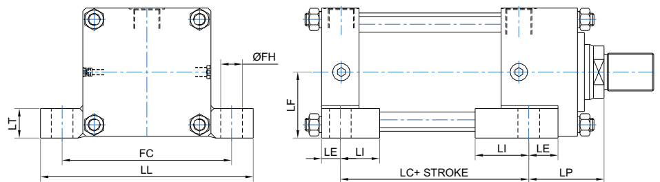
DIMENSIONAL DETAILS
