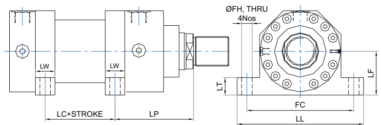
DIMENSIONAL DETAILS
