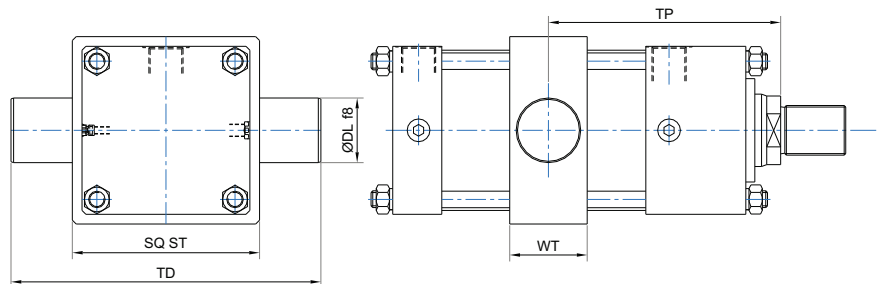
DIMENSIONAL DETAILS
